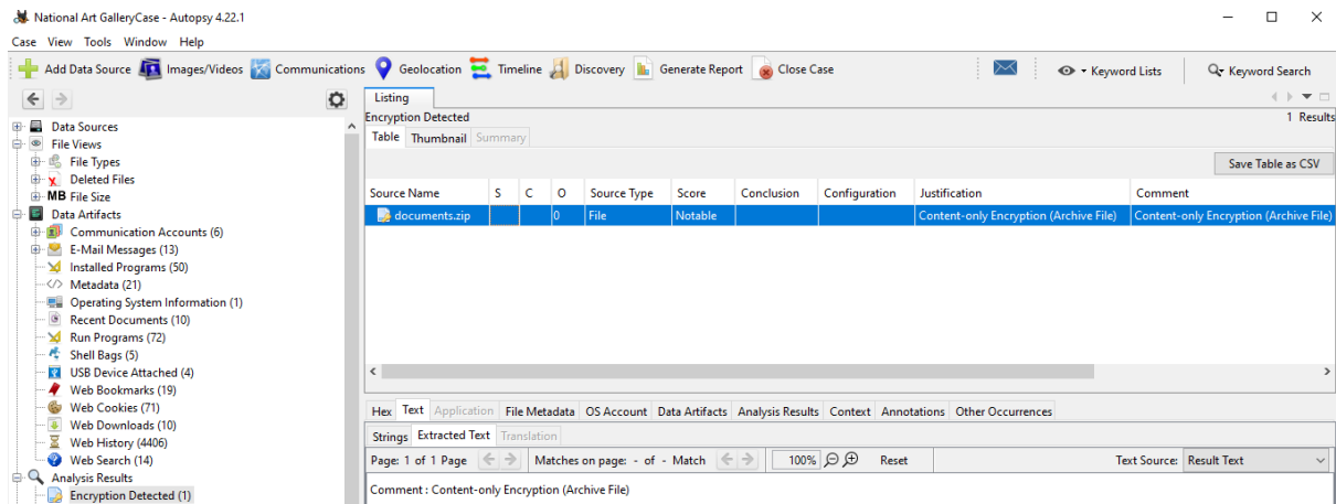
Figure 4: Encrypted zip file
